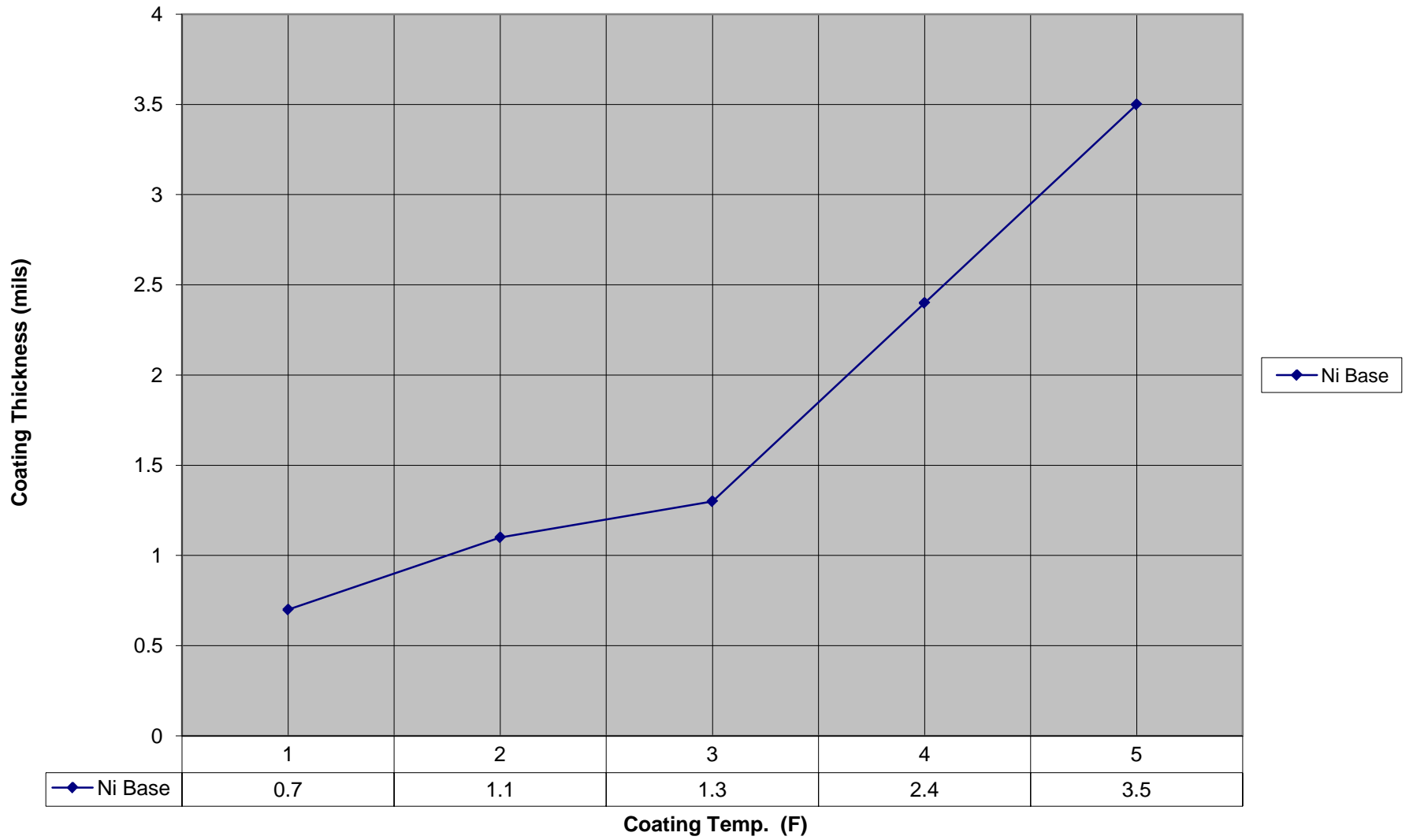
Coating Thickness vs Coating Temperature
