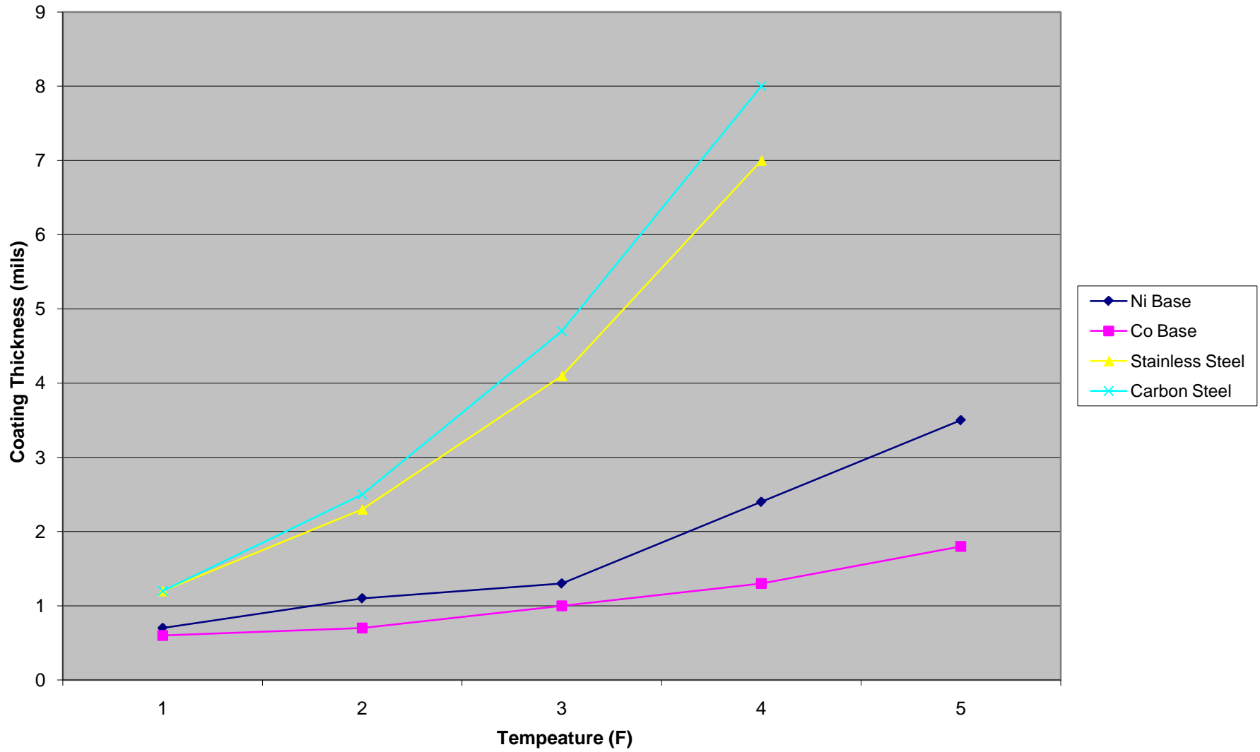
Coating Thickness vs. Coating Temperaure
