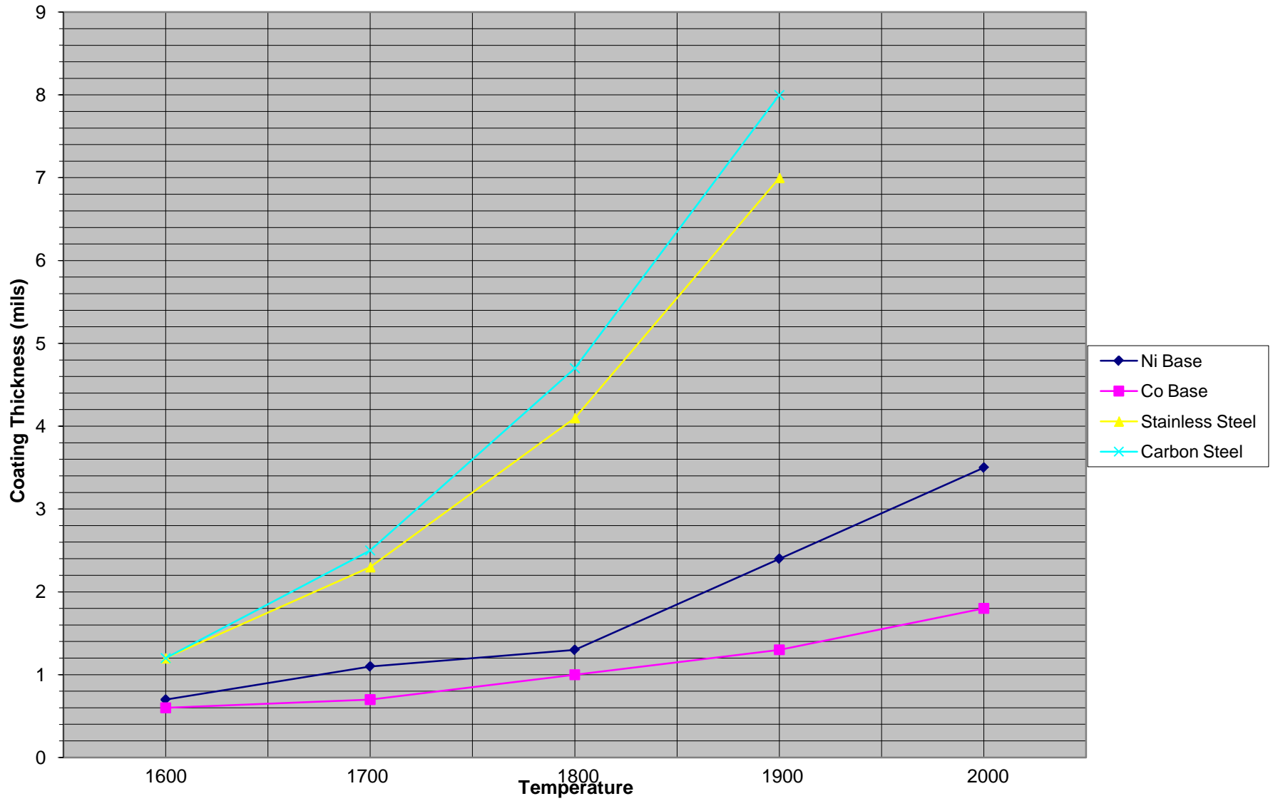
Coating Thickness vs Temperature
